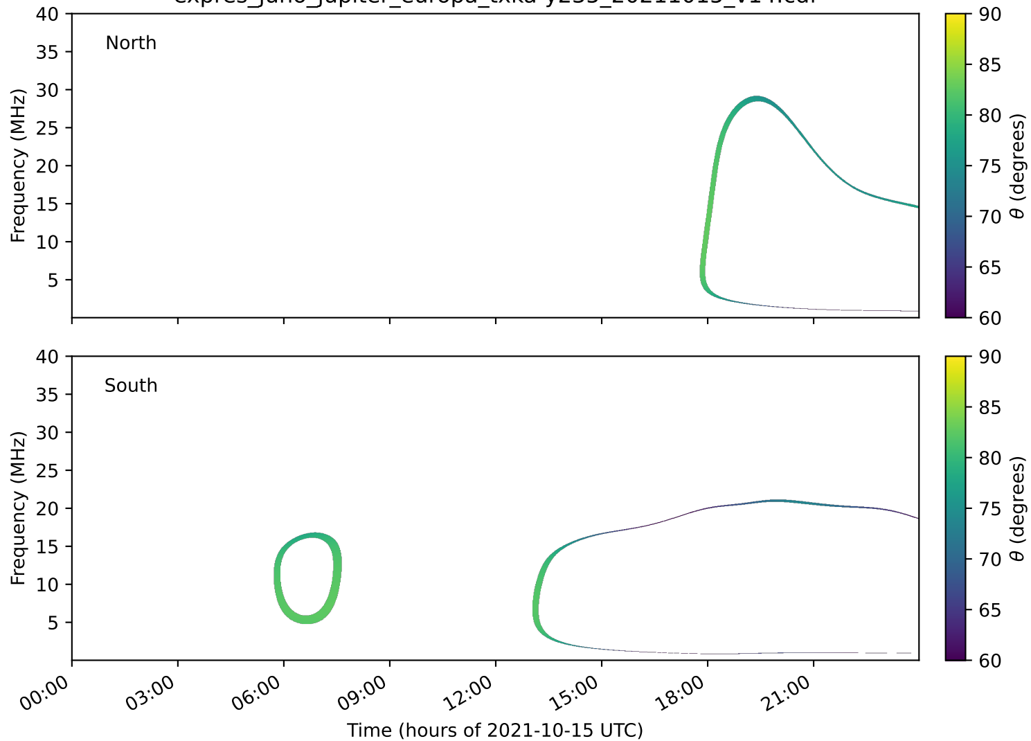
expres_juno_jupiter_europa_txka-y235_20211015_v14.cdf
