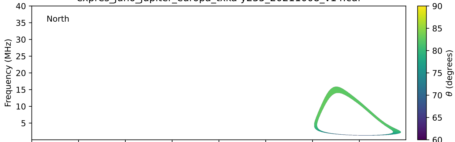
expres_juno_jupiter_europa_txka-y235_20211008_v14.cdf
