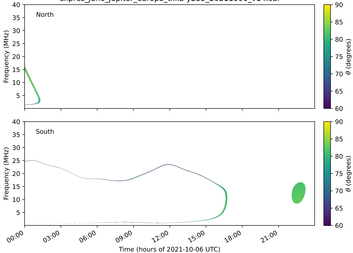
expres_juno_jupiter_europa_txka-y235_20211006_v14.cdf
