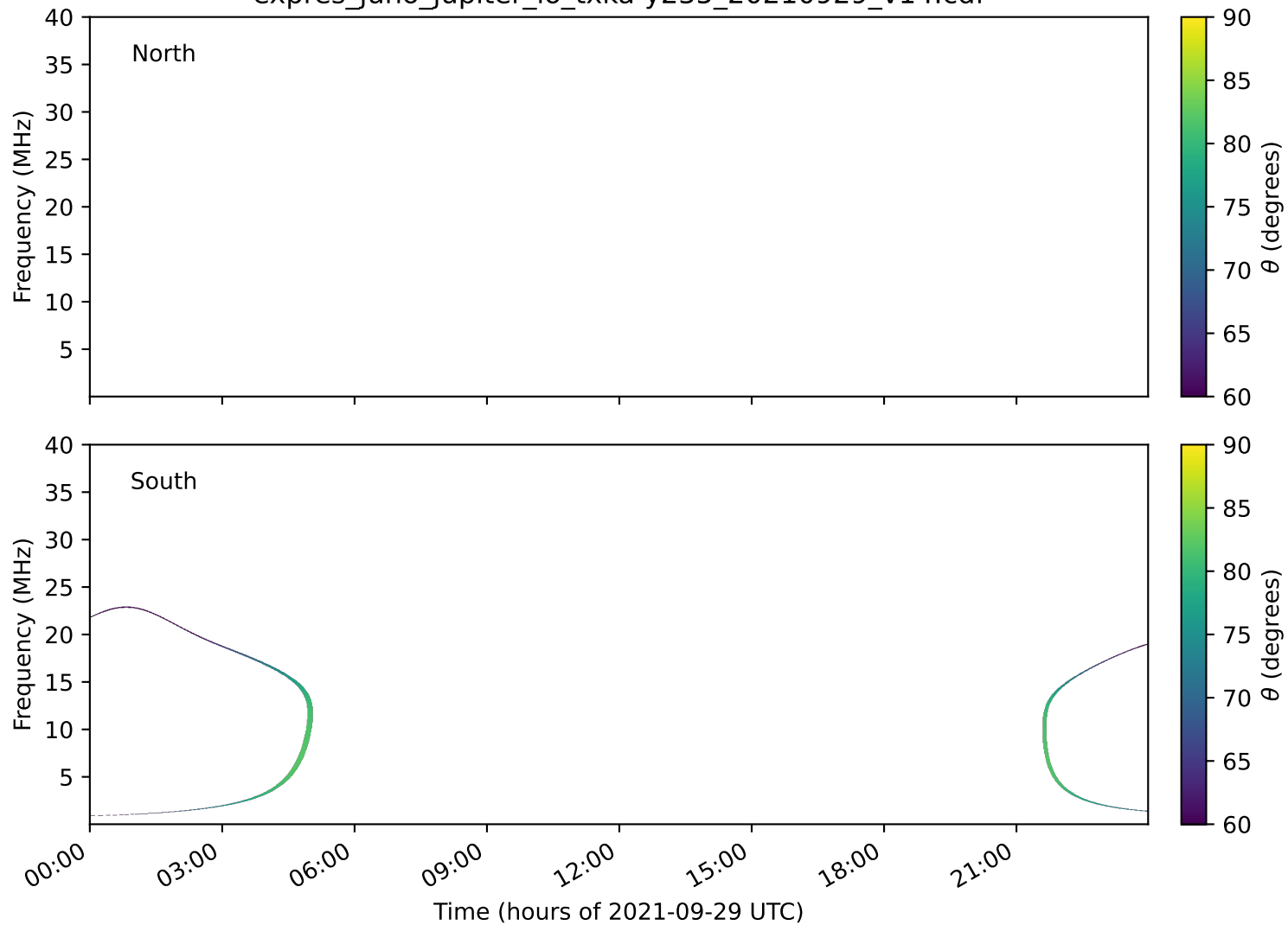
expres_juno_jupiter_io_txka-y235_20210929_v14.cdf
