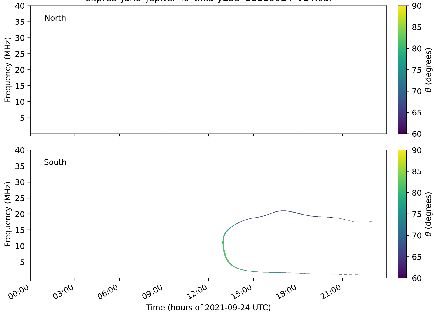
expres_juno_jupiter_io_txka-y235_20210924_v14.cdf
