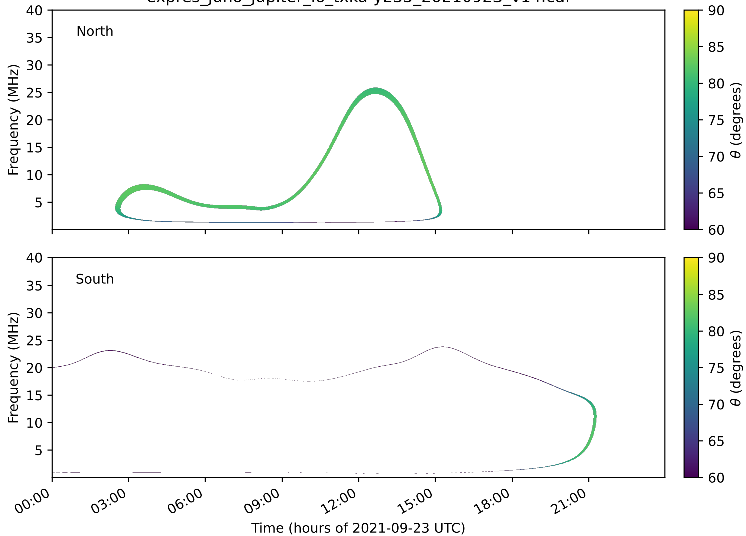
expres_juno_jupiter_io_txka-y235_20210923_v14.cdf
