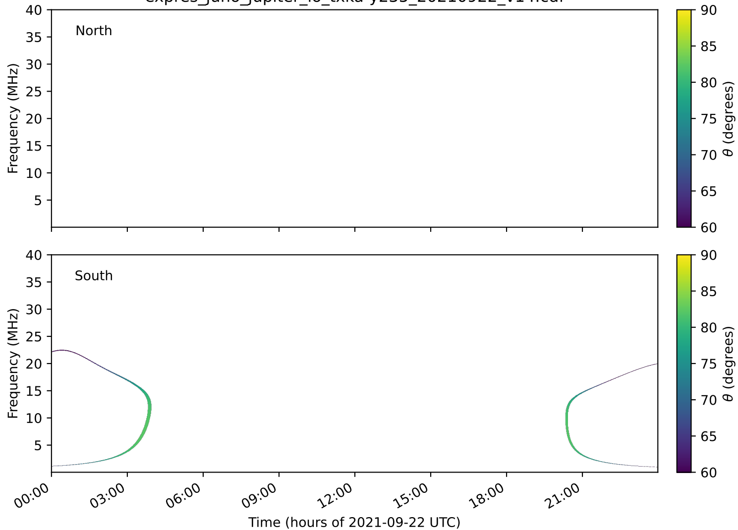
expres_juno_jupiter_io_txka-y235_20210922_v14.cdf
