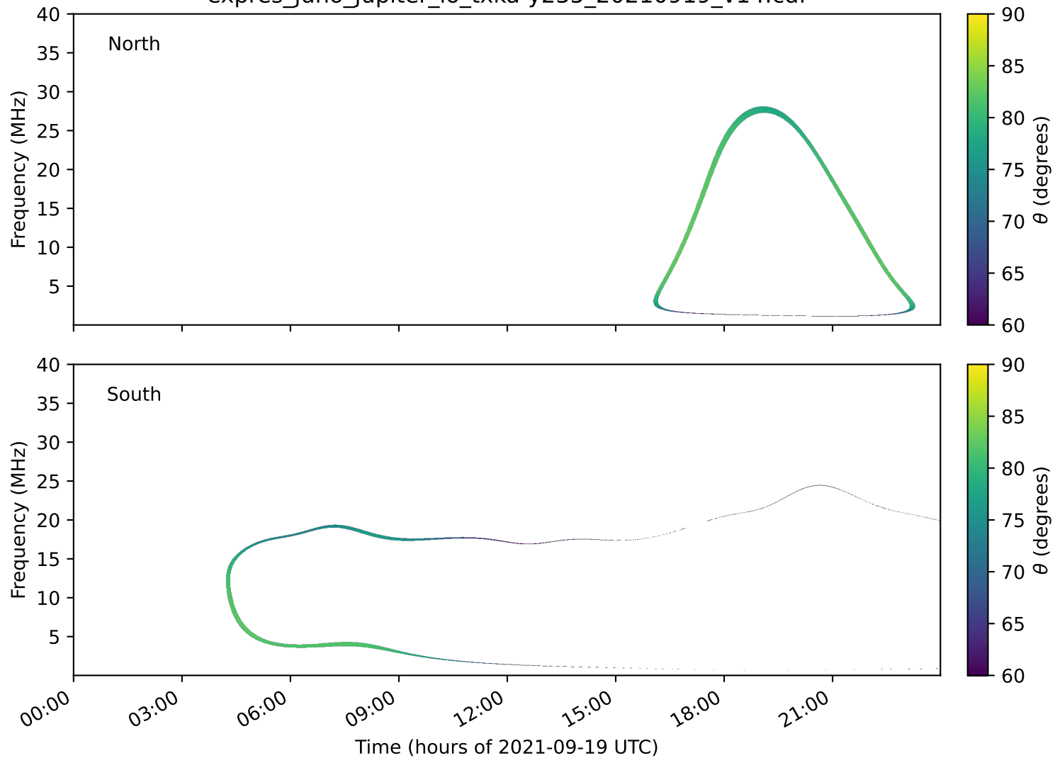
expres_juno_jupiter_io_txka-y235_20210919_v14.cdf
