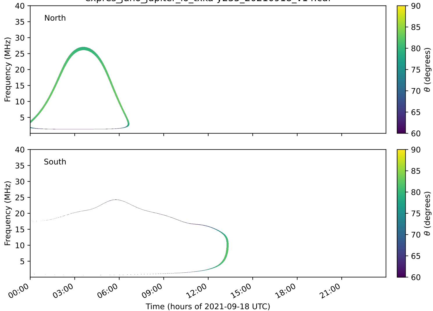
expres_juno_jupiter_io_txka-y235_20210918_v14.cdf
