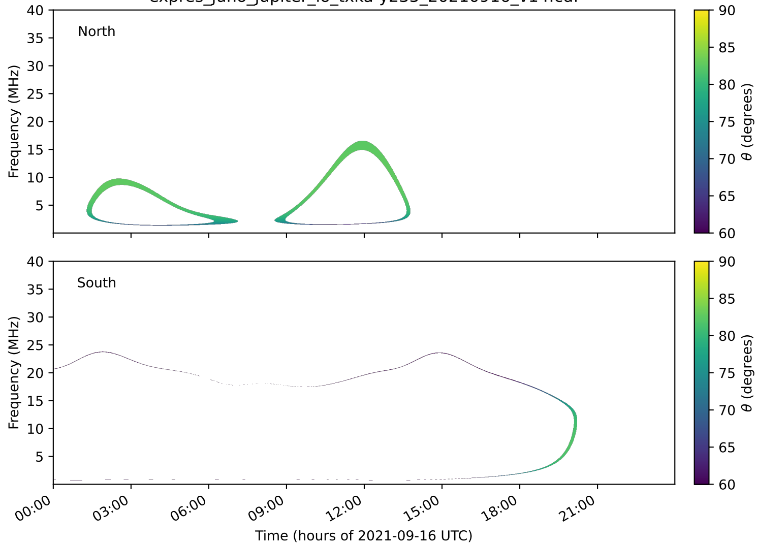
expres_juno_jupiter_io_txka-y235_20210916_v14.cdf
