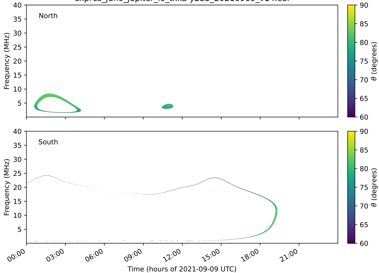
expres_juno_jupiter_io_txka-y235_20210909_v14.cdf
