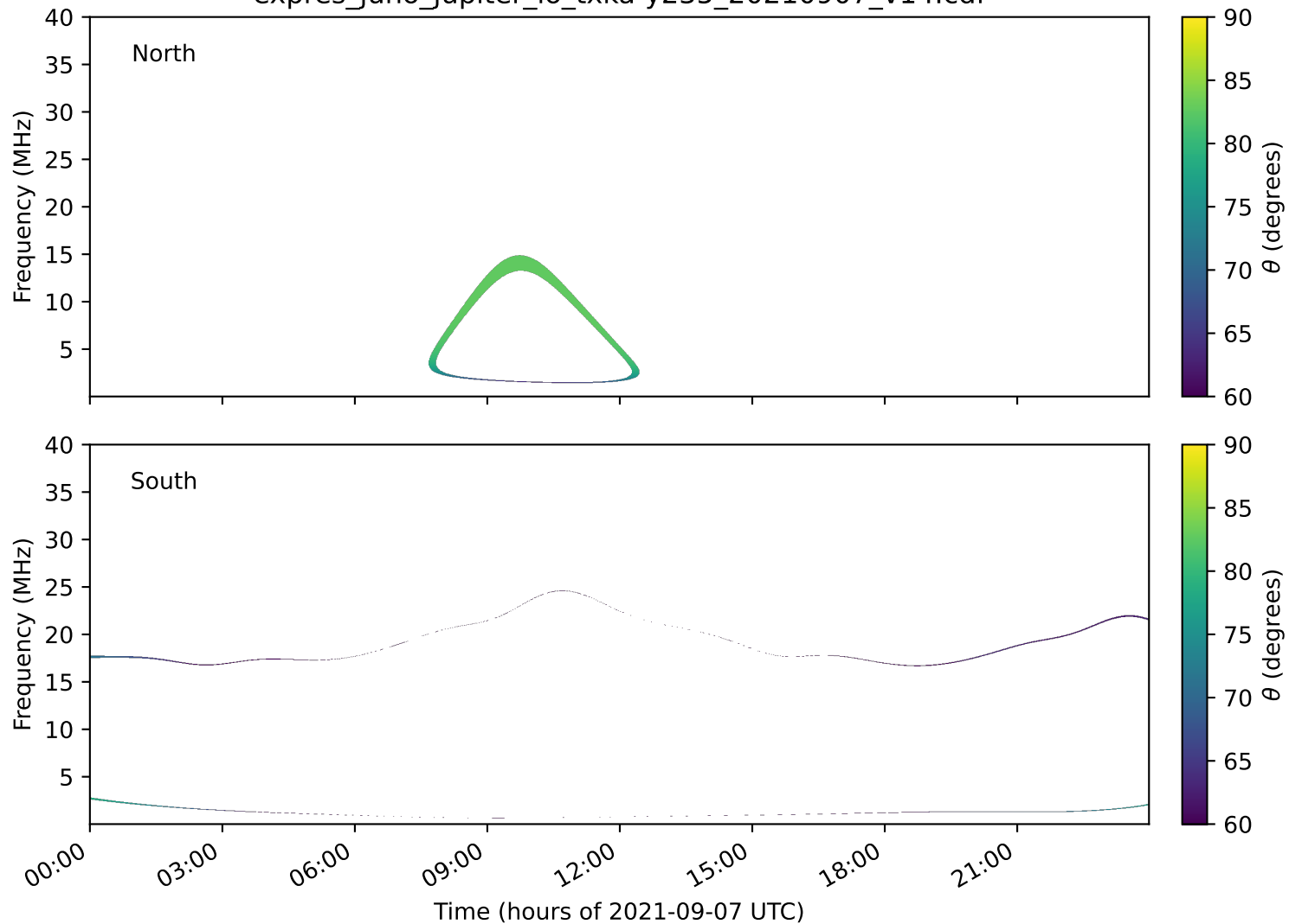
expres_juno_jupiter_io_txka-y235_20210907_v14.cdf
