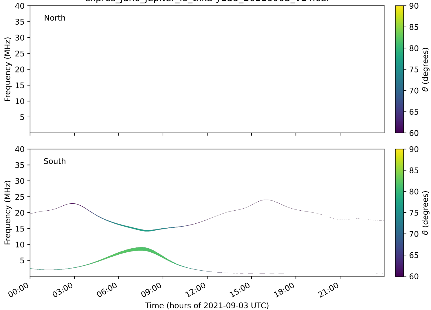
expres_juno_jupiter_io_txka-y235_20210903_v14.cdf
