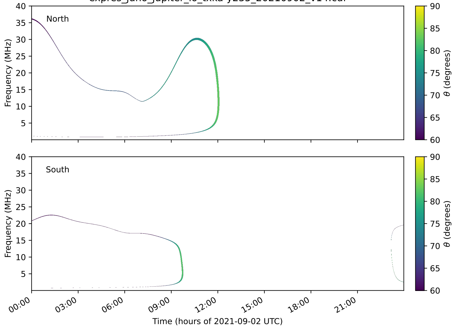
expres_juno_jupiter_io_txka-y235_20210902_v14.cdf
