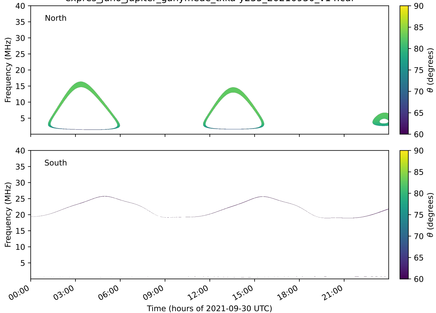
expres_juno_jupiter_ganymede_txka-y235_20210930_v14.cdf
