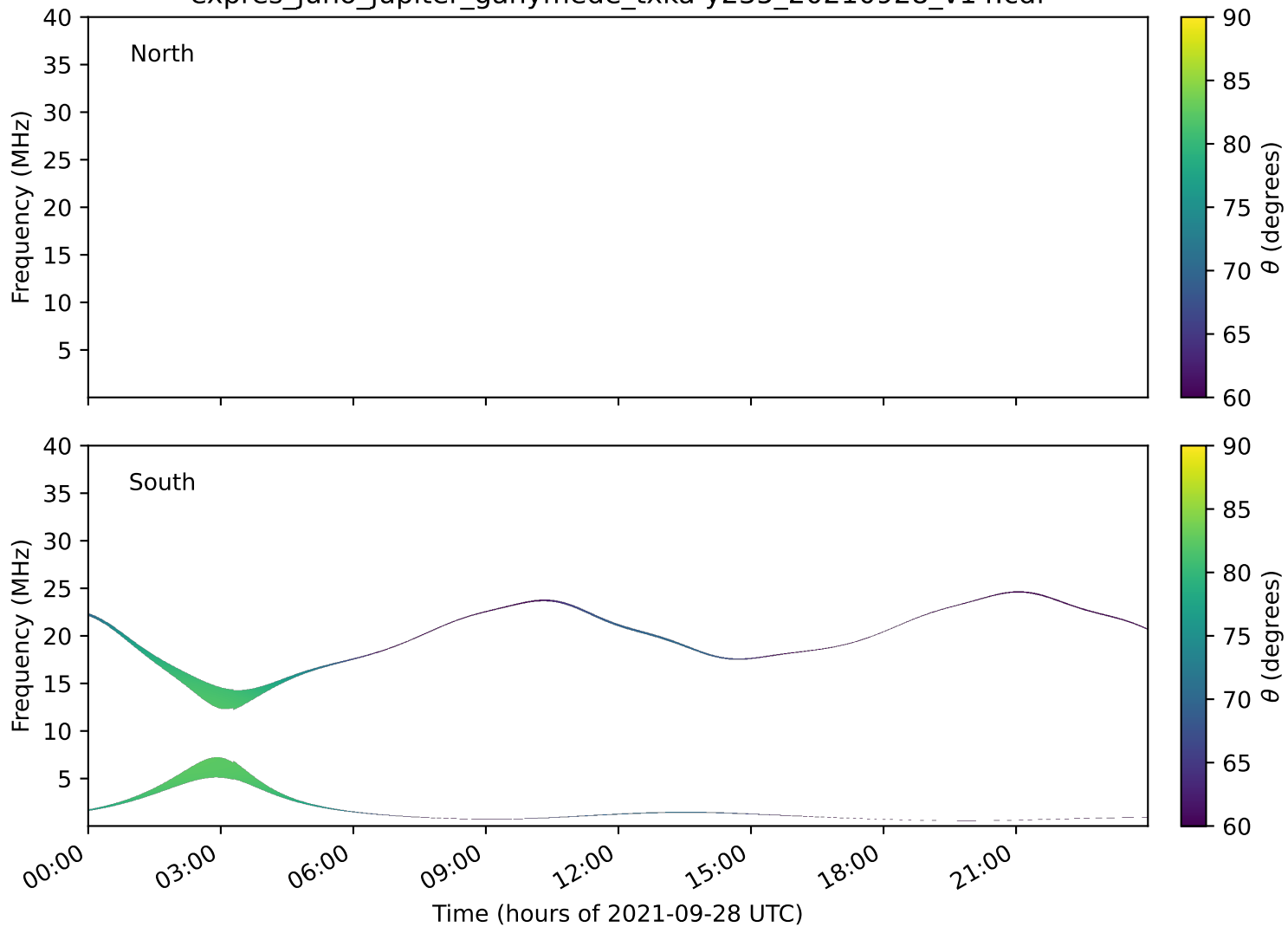
expres_juno_jupiter_ganymede_txka-y235_20210928_v14.cdf
