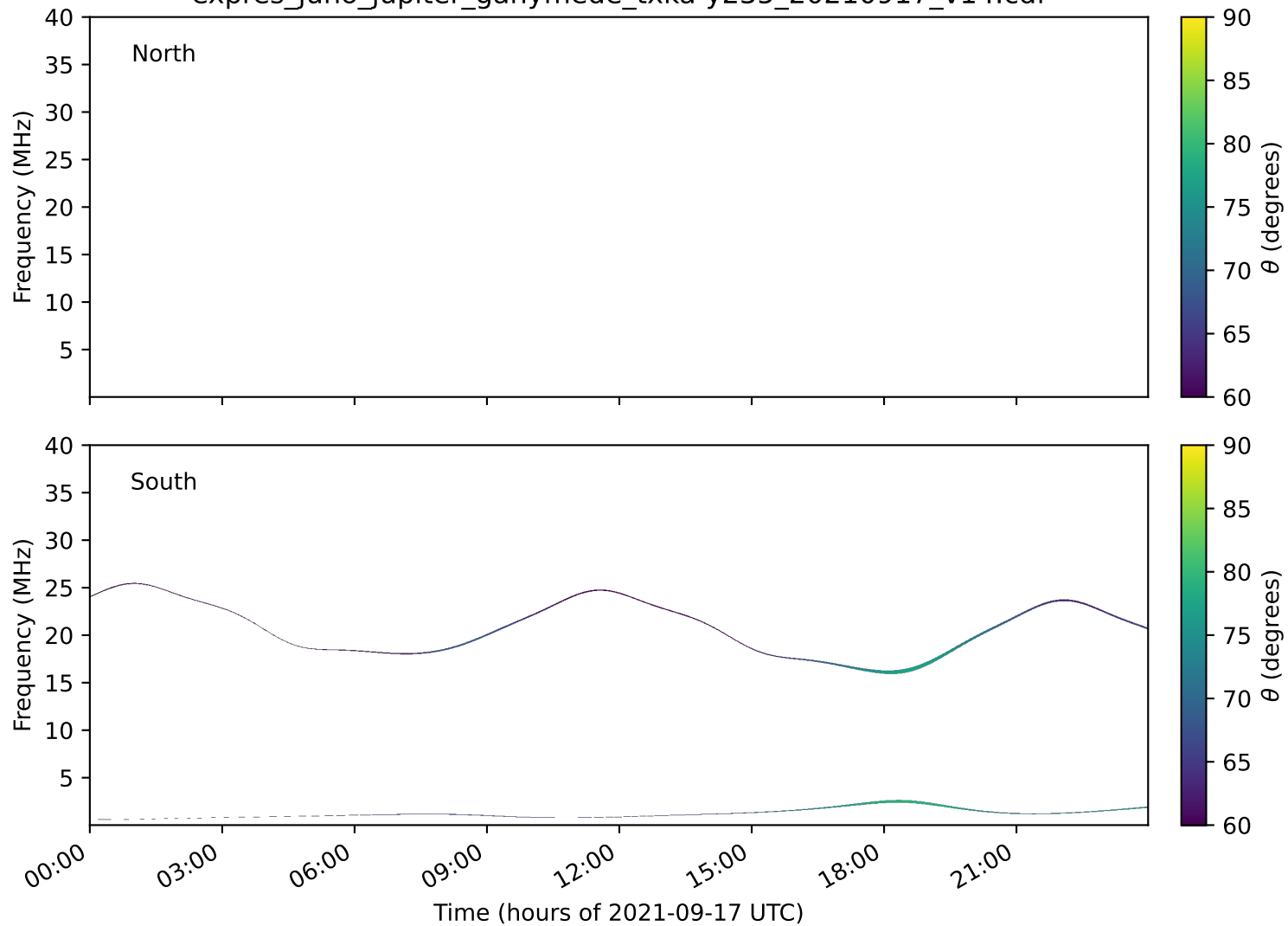
expres_juno_jupiter_ganymede_txka-y235_20210917_v14.cdf
