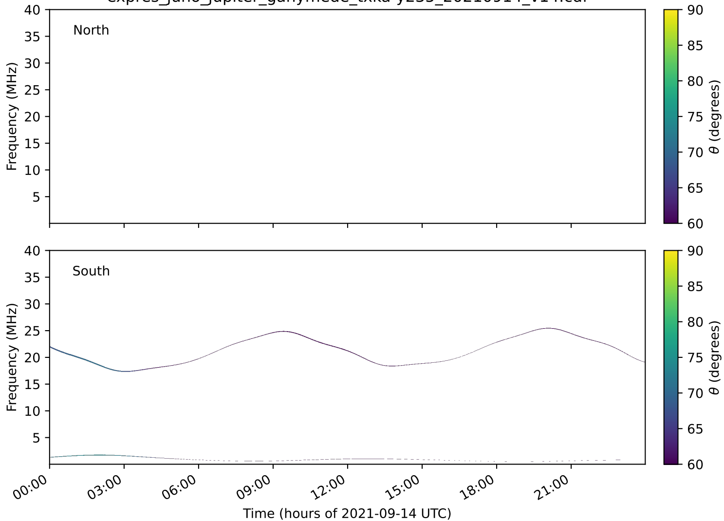
expres_juno_jupiter_ganymede_txka-y235_20210914_v14.cdf
