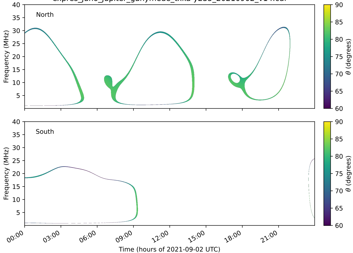
expres_juno_jupiter_ganymede_txka-y235_20210902_v14.cdf
