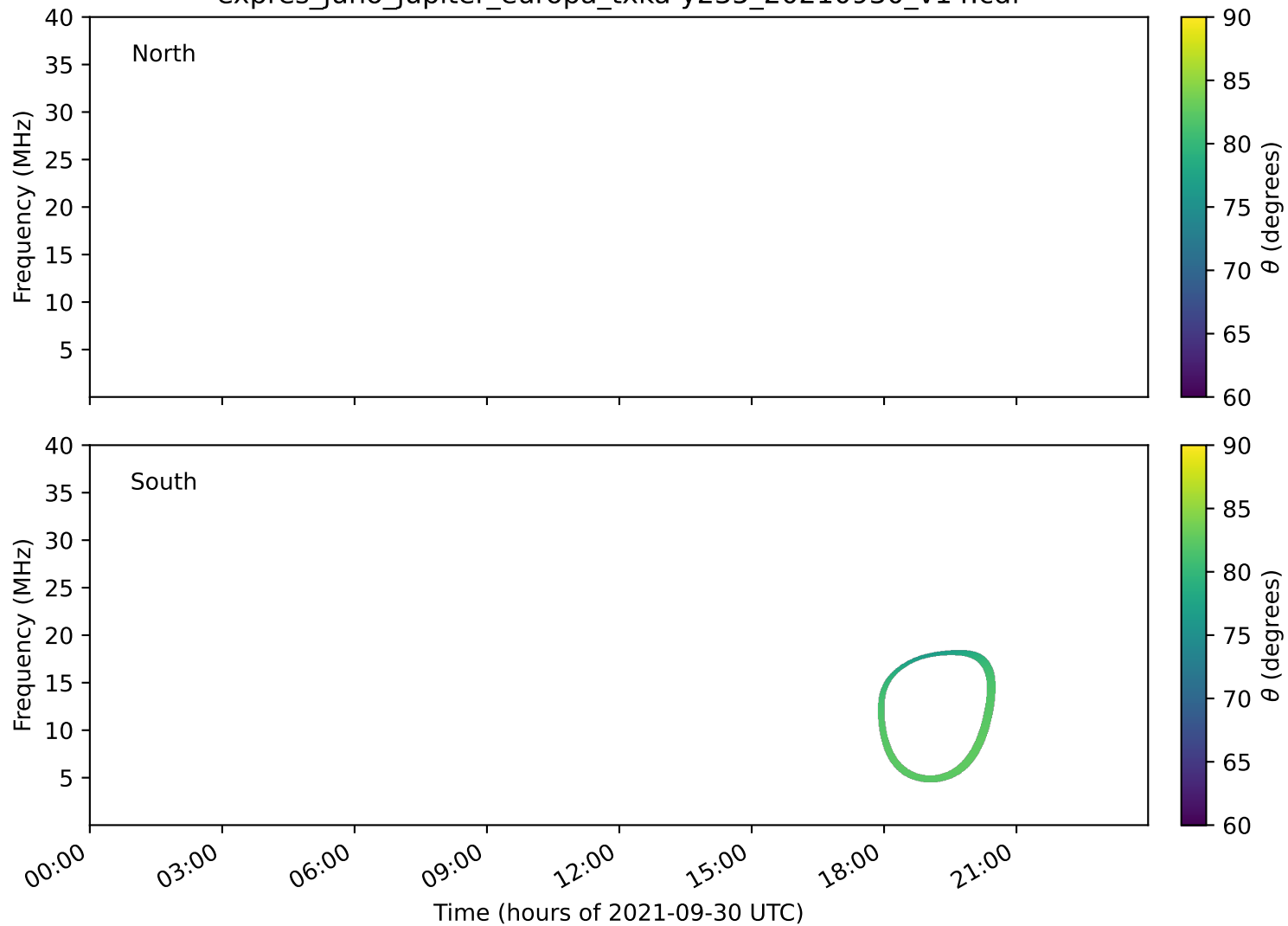
expres_juno_jupiter_europa_txka-y235_20210930_v14.cdf
