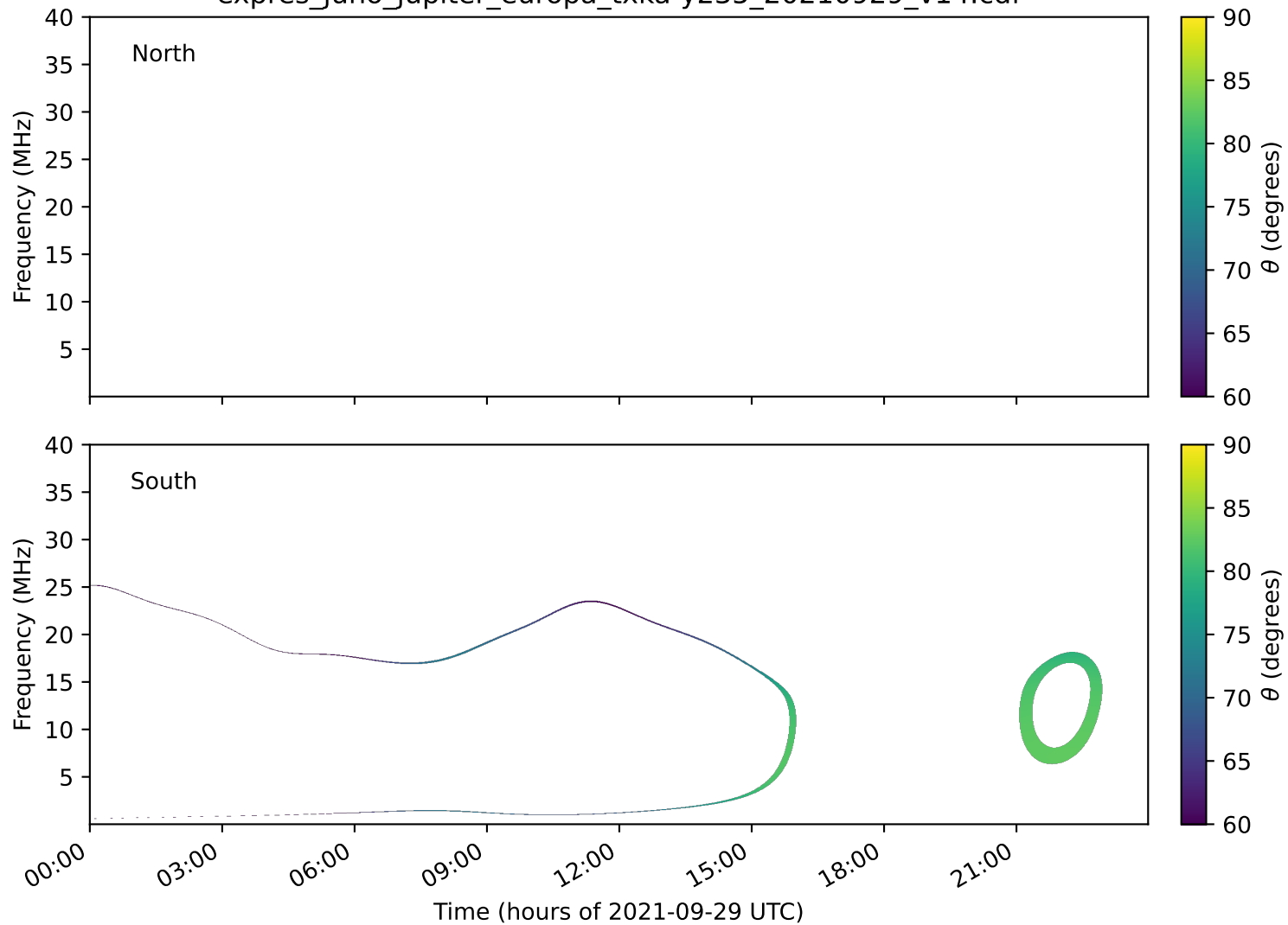
expres_juno_jupiter_europa_txka-y235_20210929_v14.cdf
