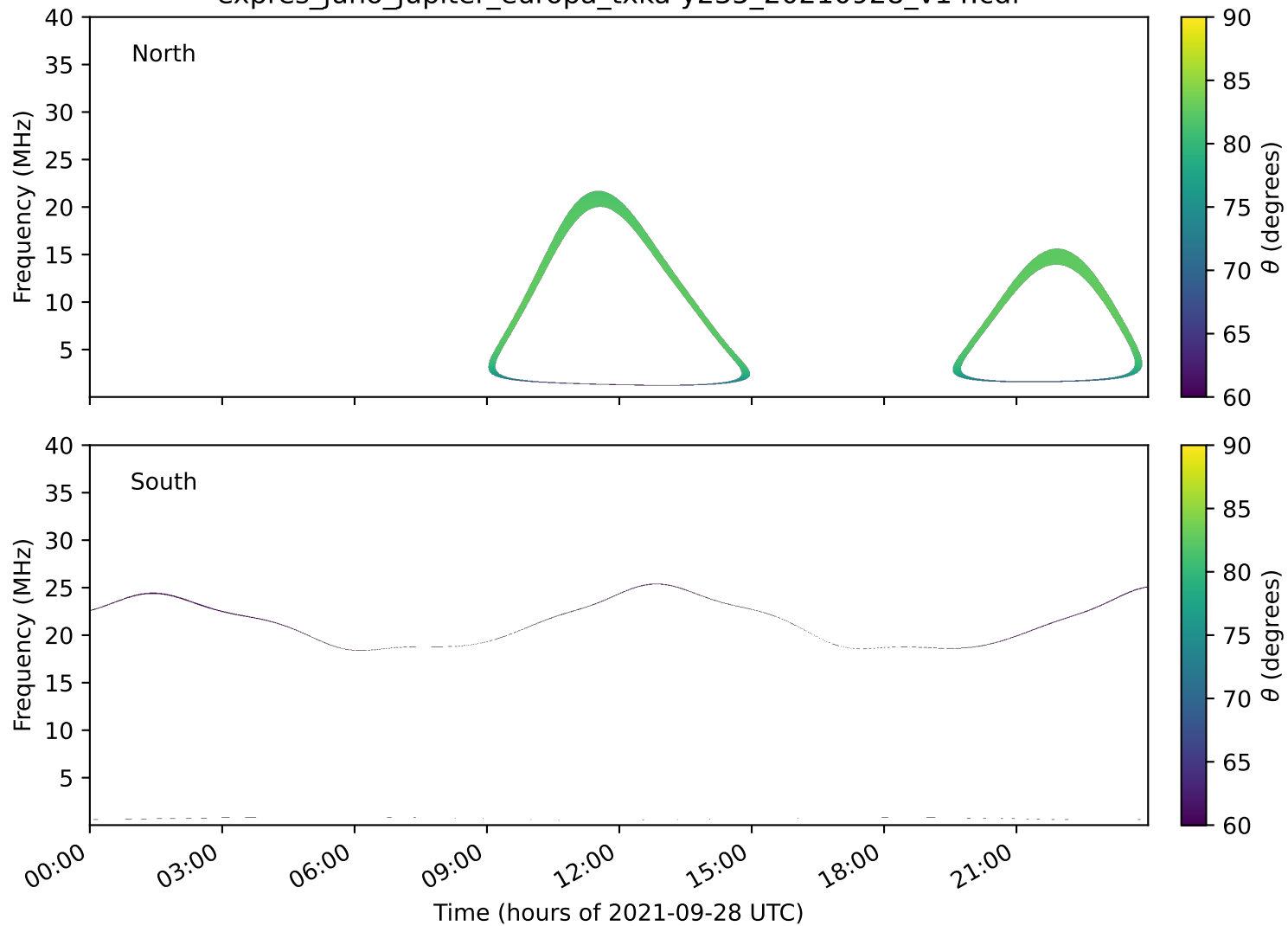
expres_juno_jupiter_europa_txka-y235_20210928_v14.cdf
