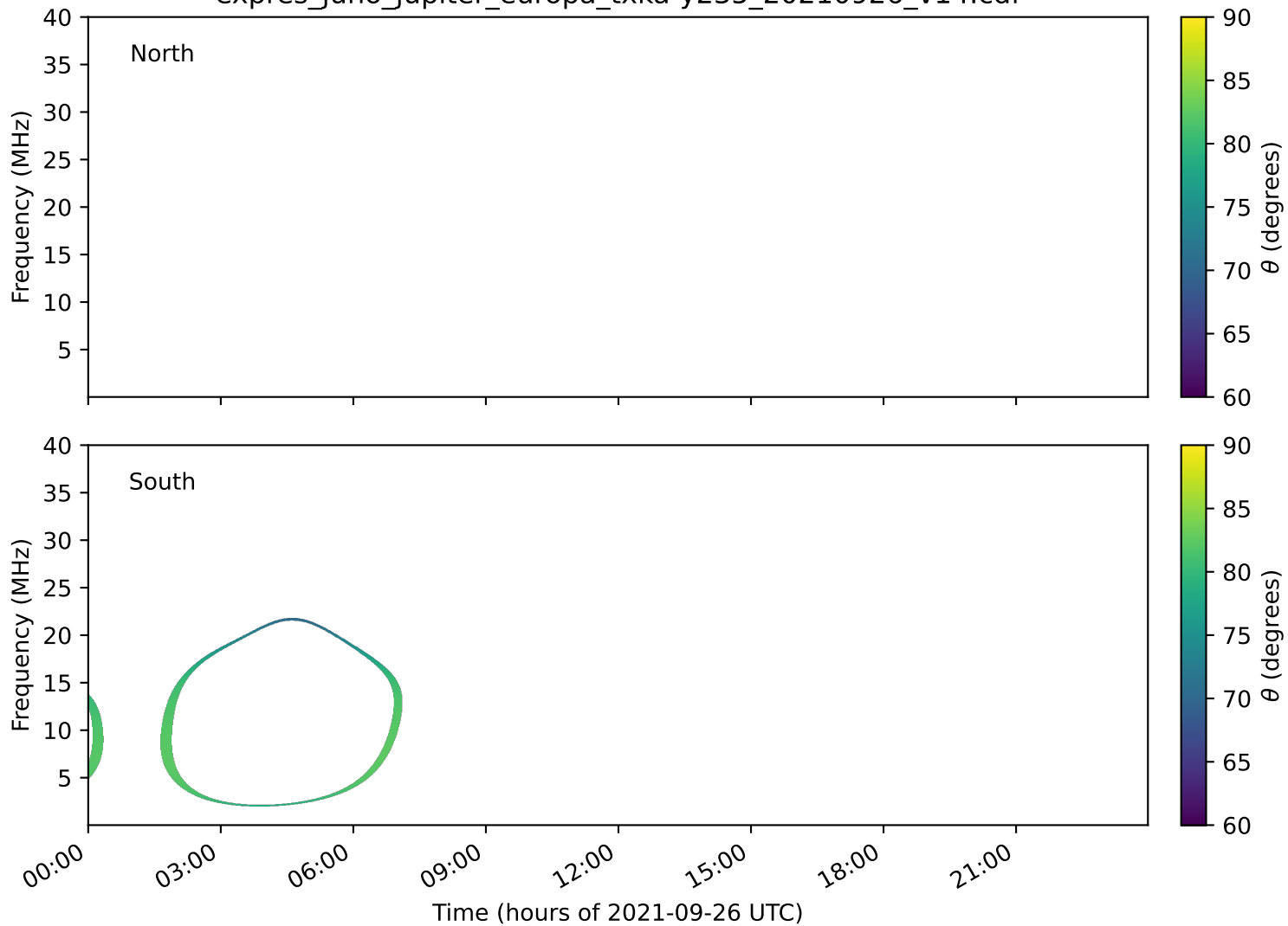
expres_juno_jupiter_europa_txka-y235_20210926_v14.cdf
