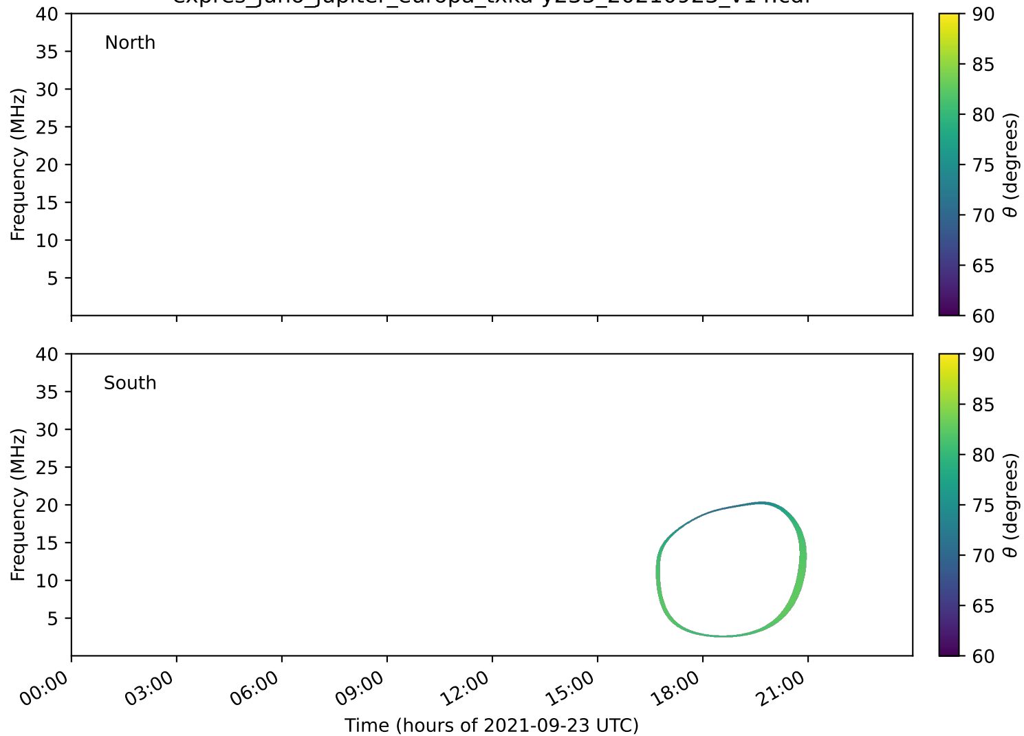
expres_juno_jupiter_europa_txka-y235_20210923_v14.cdf
