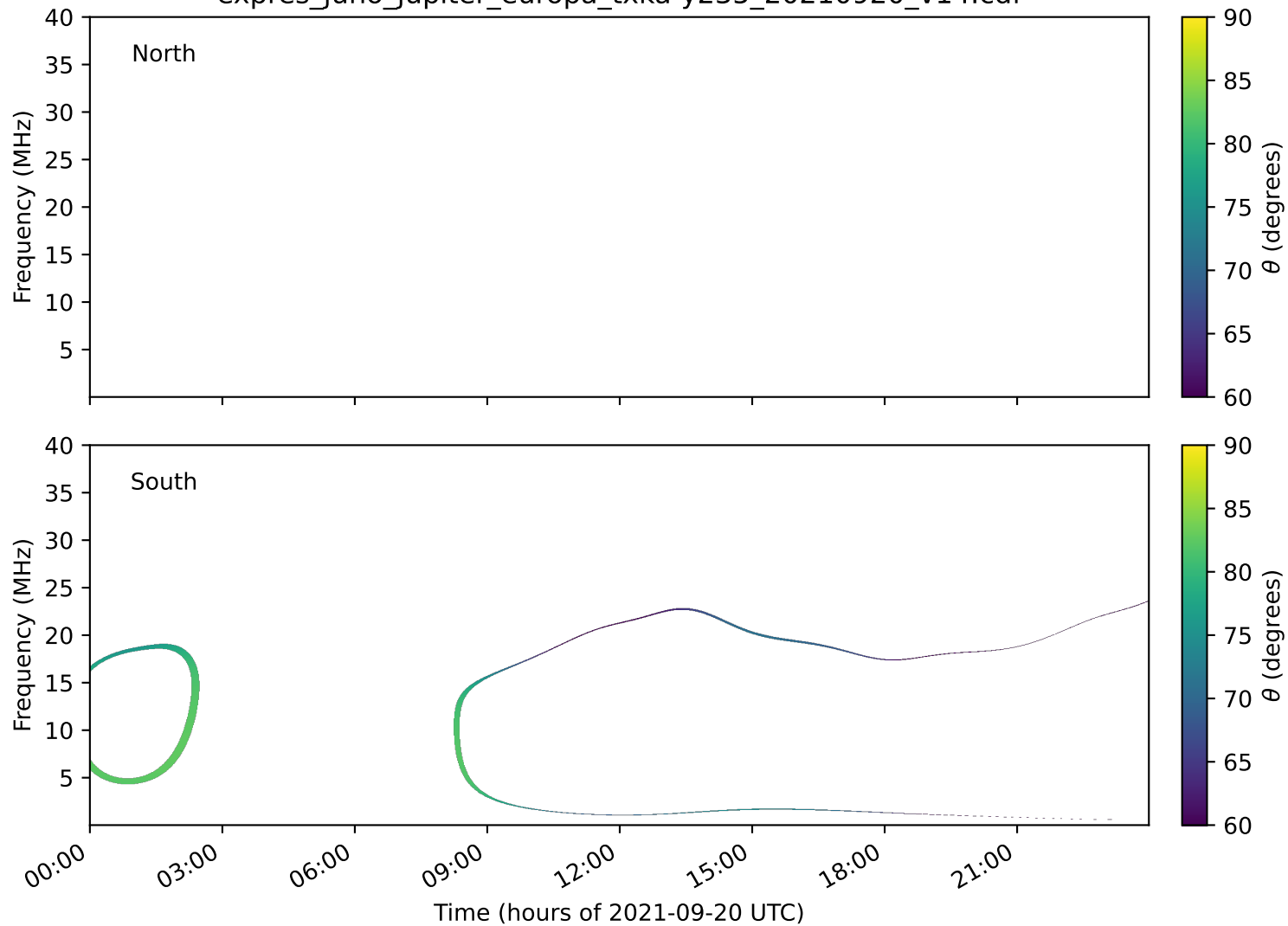
expres_juno_jupiter_europa_txka-y235_20210920_v14.cdf
