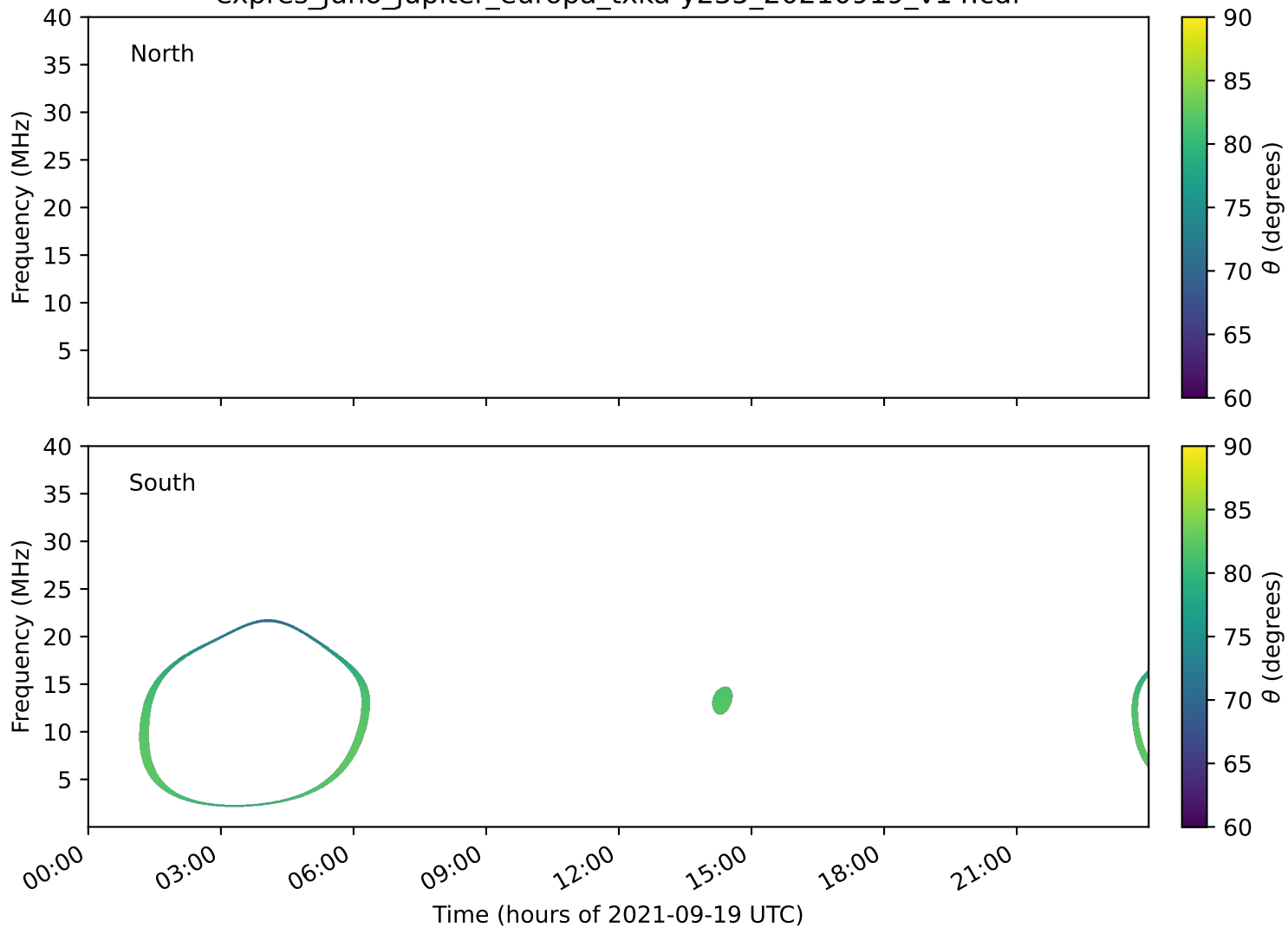
expres_juno_jupiter_europa_txka-y235_20210919_v14.cdf
