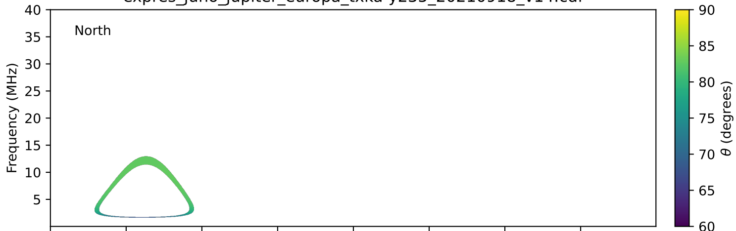
expres_juno_jupiter_europa_txka-y235_20210918_v14.cdf
