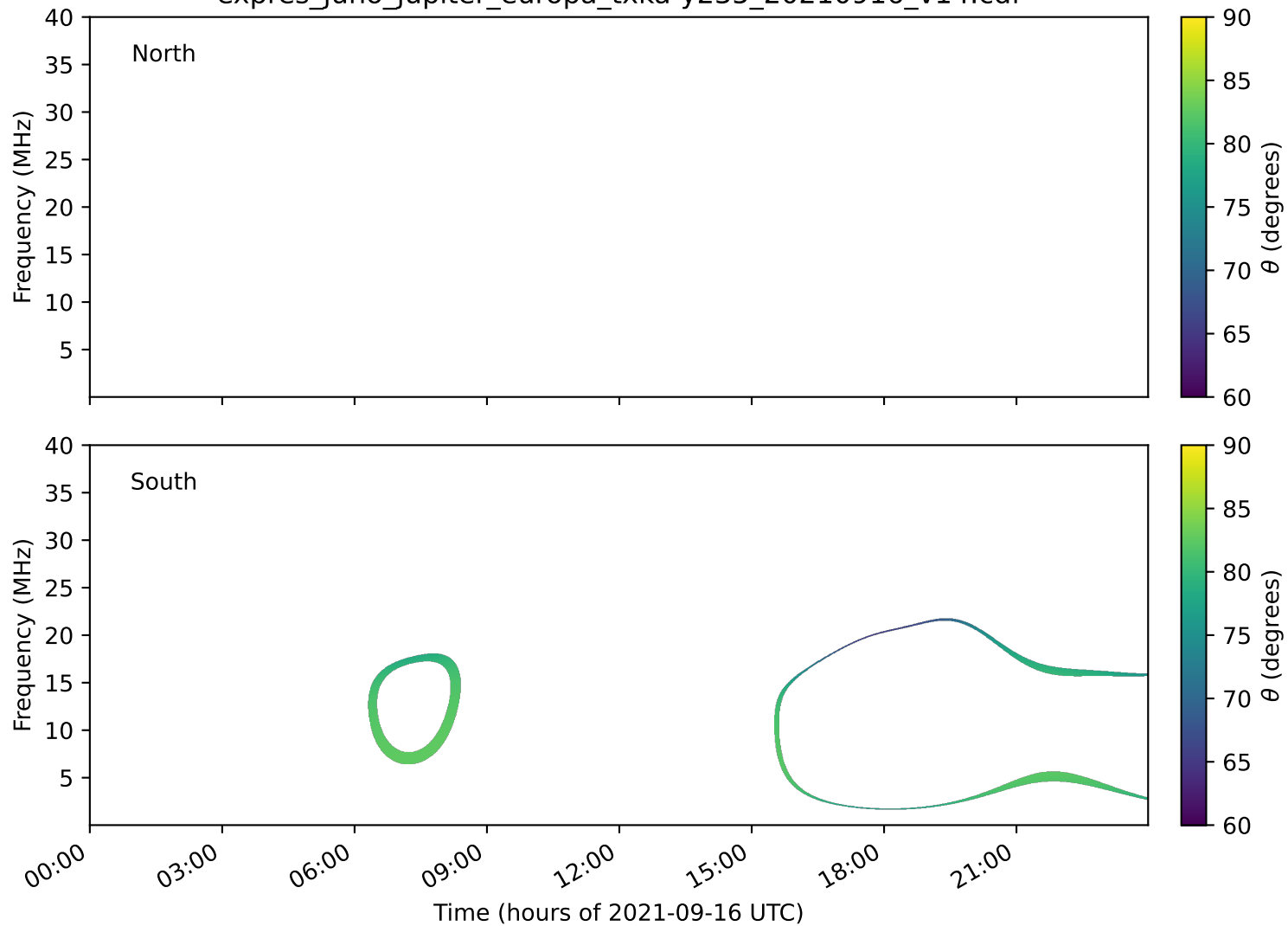
expres_juno_jupiter_europa_txka-y235_20210916_v14.cdf
