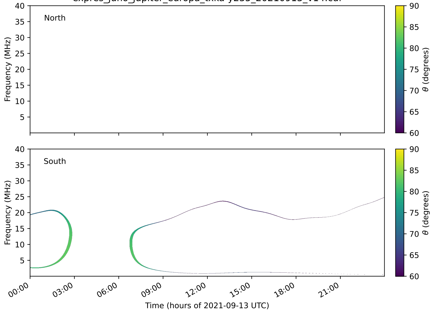
expres_juno_jupiter_europa_txka-y235_20210913_v14.cdf
