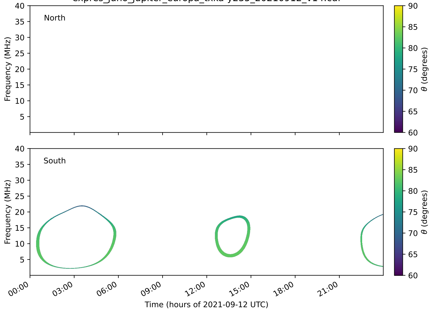
expres_juno_jupiter_europa_txka-y235_20210912_v14.cdf
