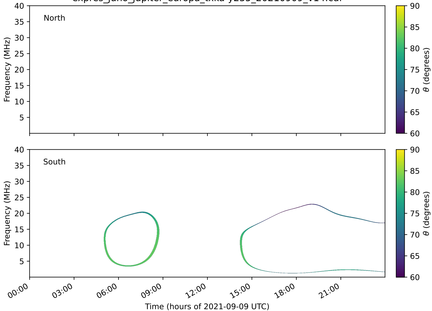
expres_juno_jupiter_europa_txka-y235_20210909_v14.cdf
