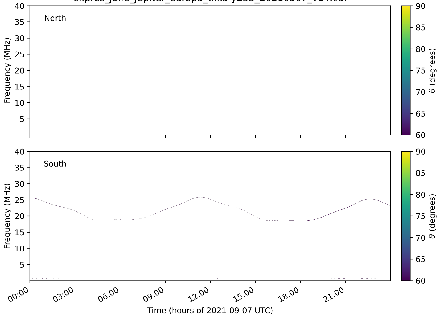
expres_juno_jupiter_europa_txka-y235_20210907_v14.cdf
