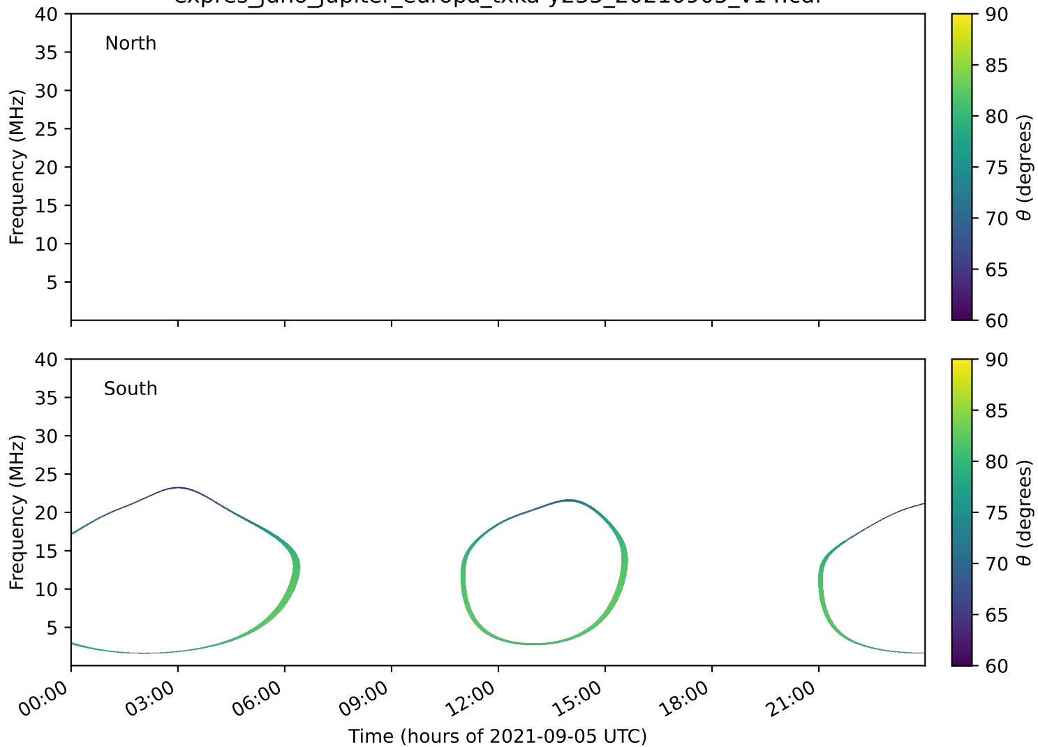
expres_juno_jupiter_europa_txka-y235_20210905_v14.cdf
