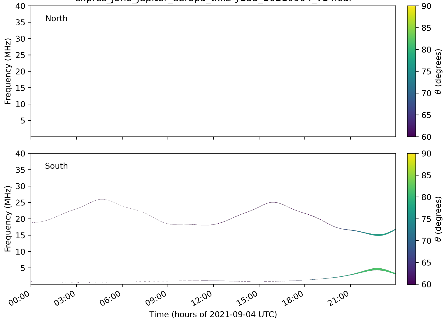
expres_juno_jupiter_europa_txka-y235_20210904_v14.cdf
