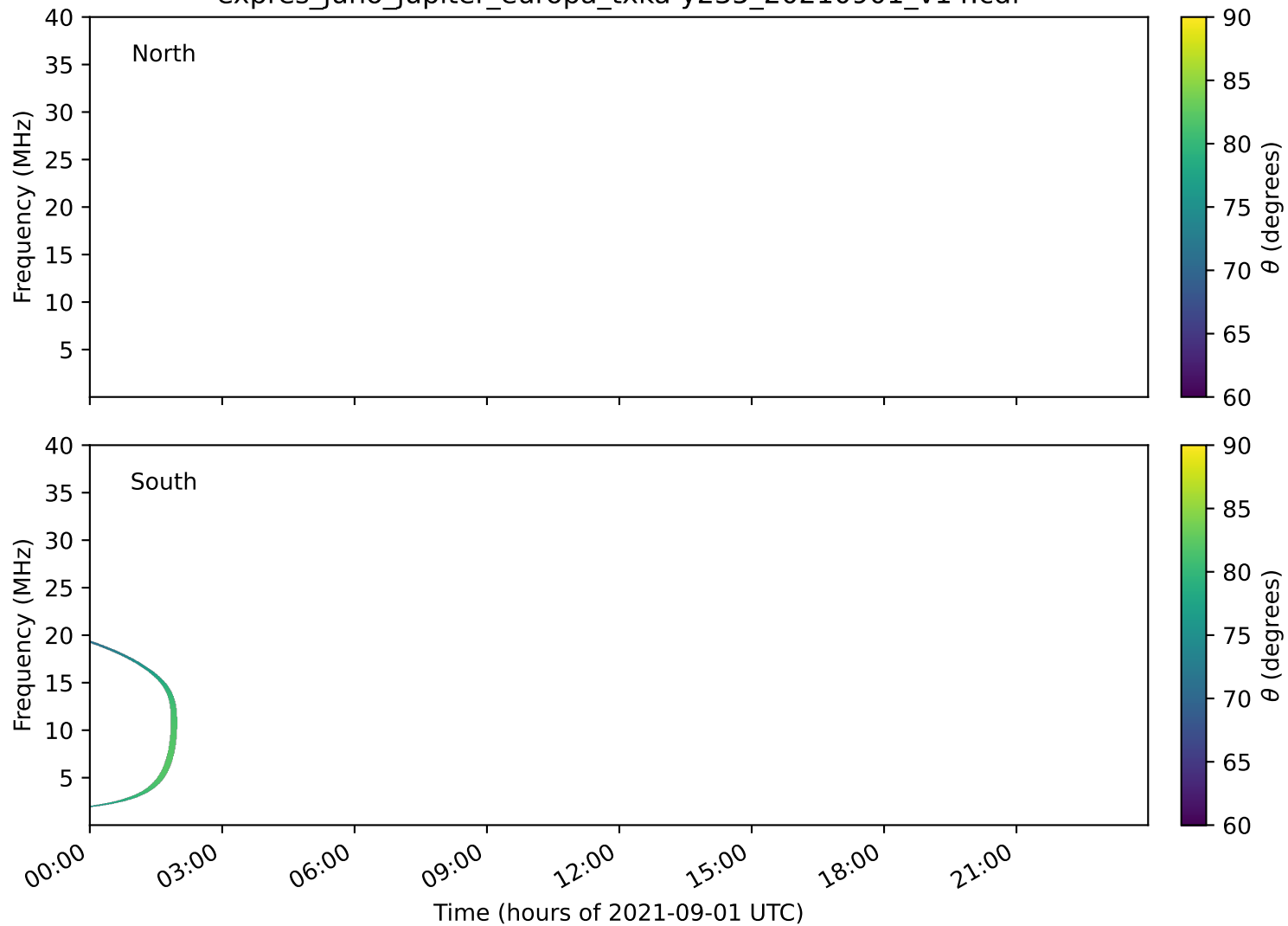
expres_juno_jupiter_europa_txka-y235_20210901_v14.cdf
