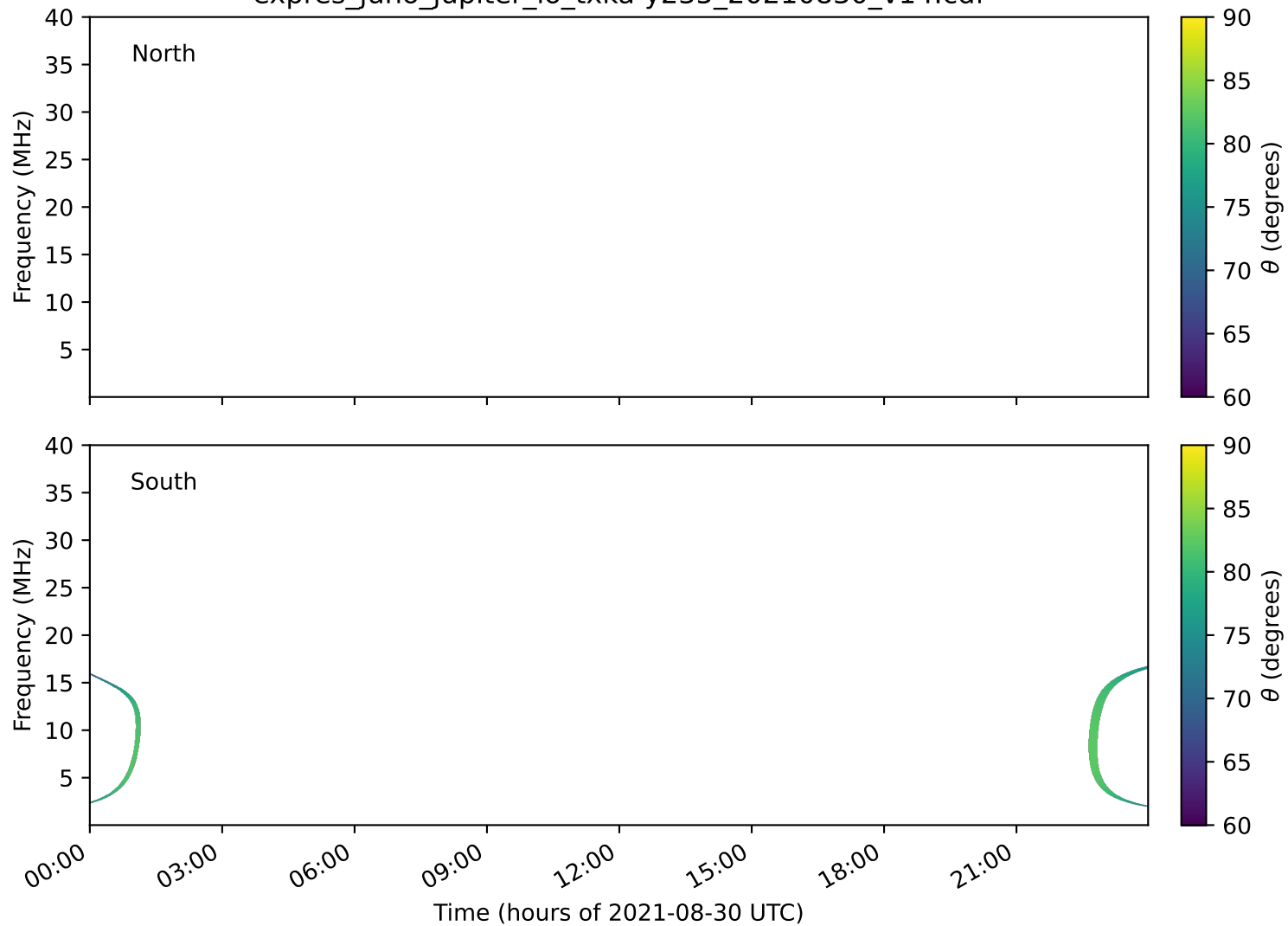
expres_juno_jupiter_io_txka-y235_20210830_v14.cdf
