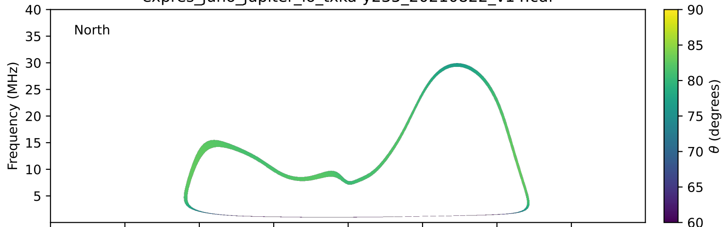
expres_juno_jupiter_io_txka-y235_20210822_v14.cdf
