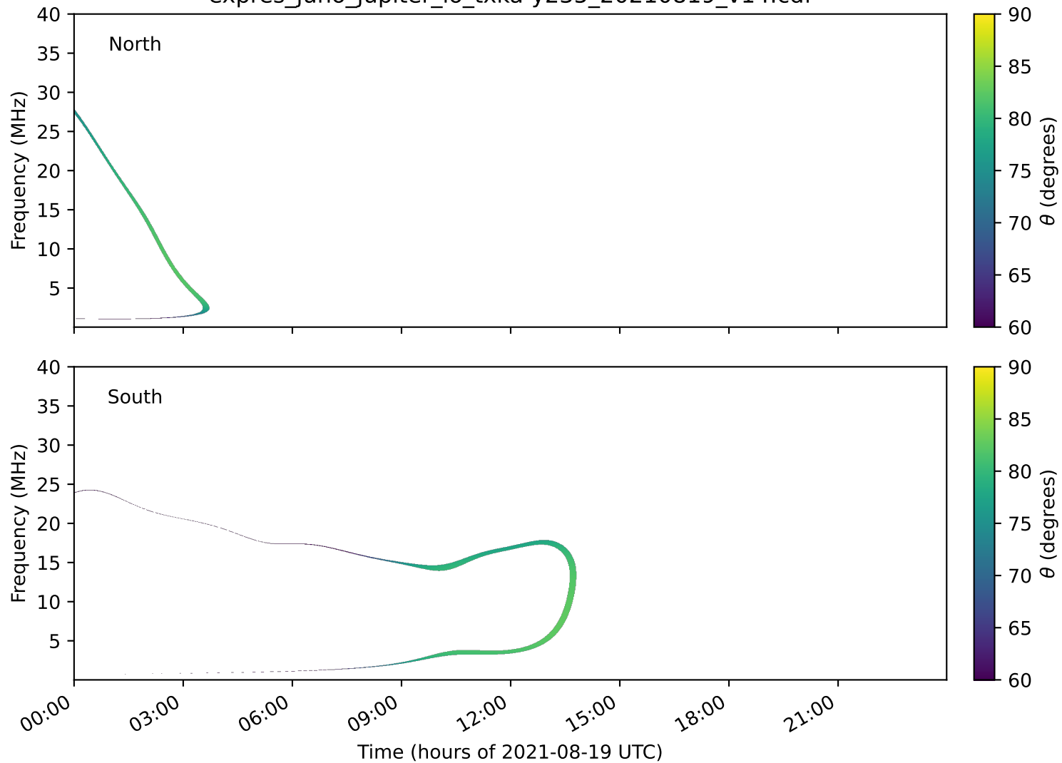
expres_juno_jupiter_io_txka-y235_20210819_v14.cdf
