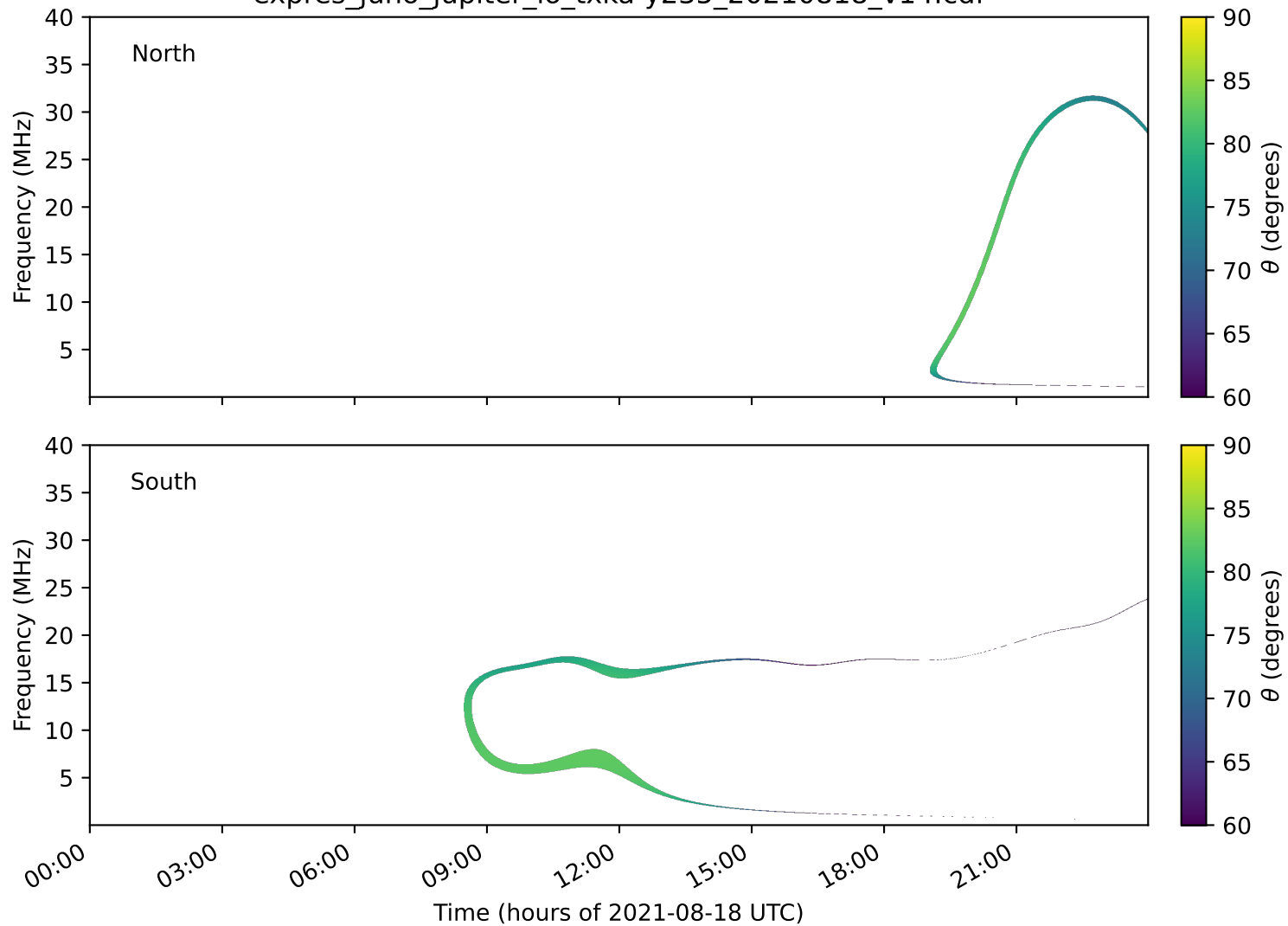
expres_juno_jupiter_io_txka-y235_20210818_v14.cdf
