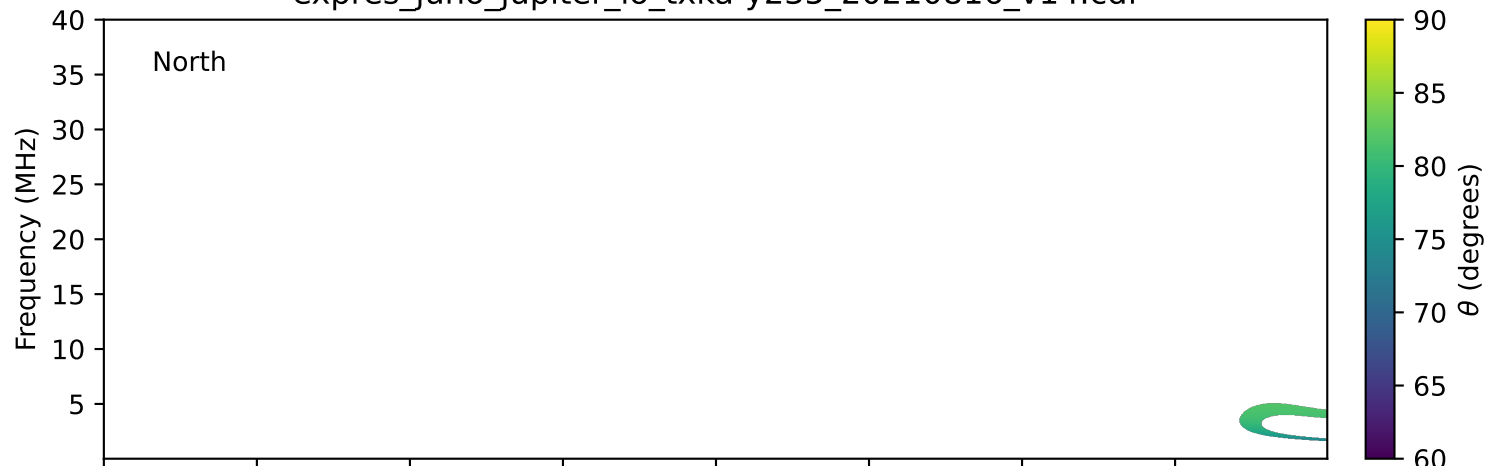
expres_juno_jupiter_io_txka-y235_20210816_v14.cdf
