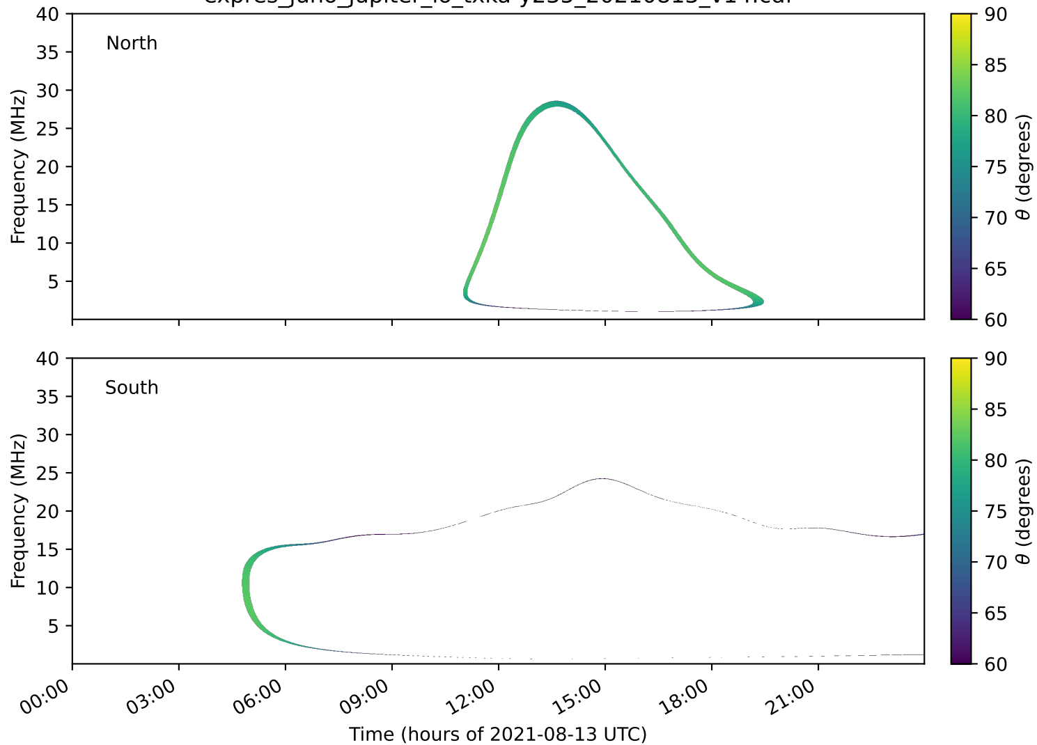
expres_juno_jupiter_io_txka-y235_20210813_v14.cdf
