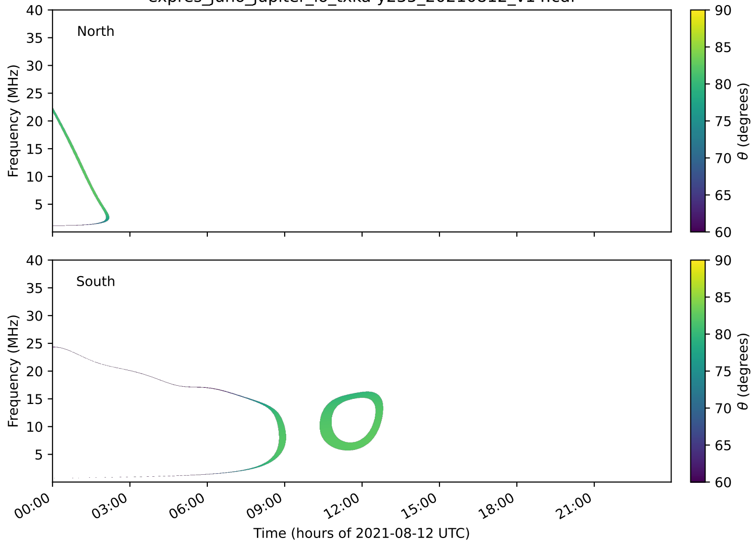
expres_juno_jupiter_io_txka-y235_20210812_v14.cdf
