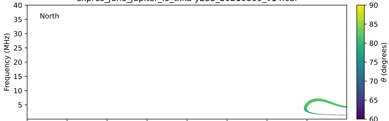
expres_juno_jupiter_io_txka-y235_20210809_v14.cdf
