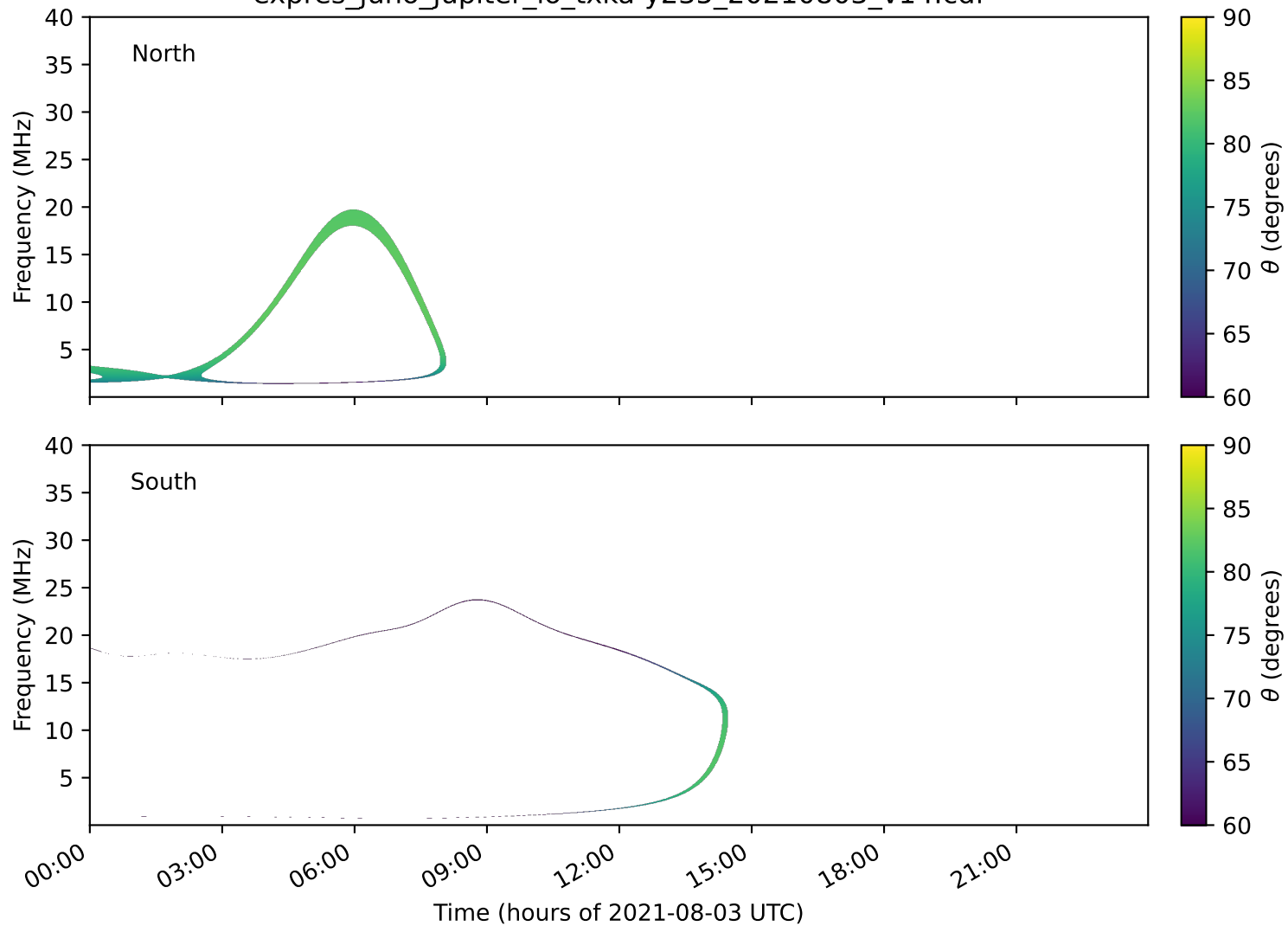
expres_juno_jupiter_io_txka-y235_20210803_v14.cdf
