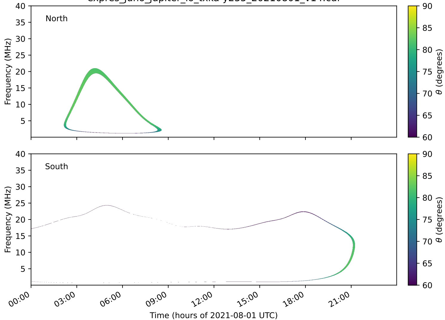
expres_juno_jupiter_io_txka-y235_20210801_v14.cdf
