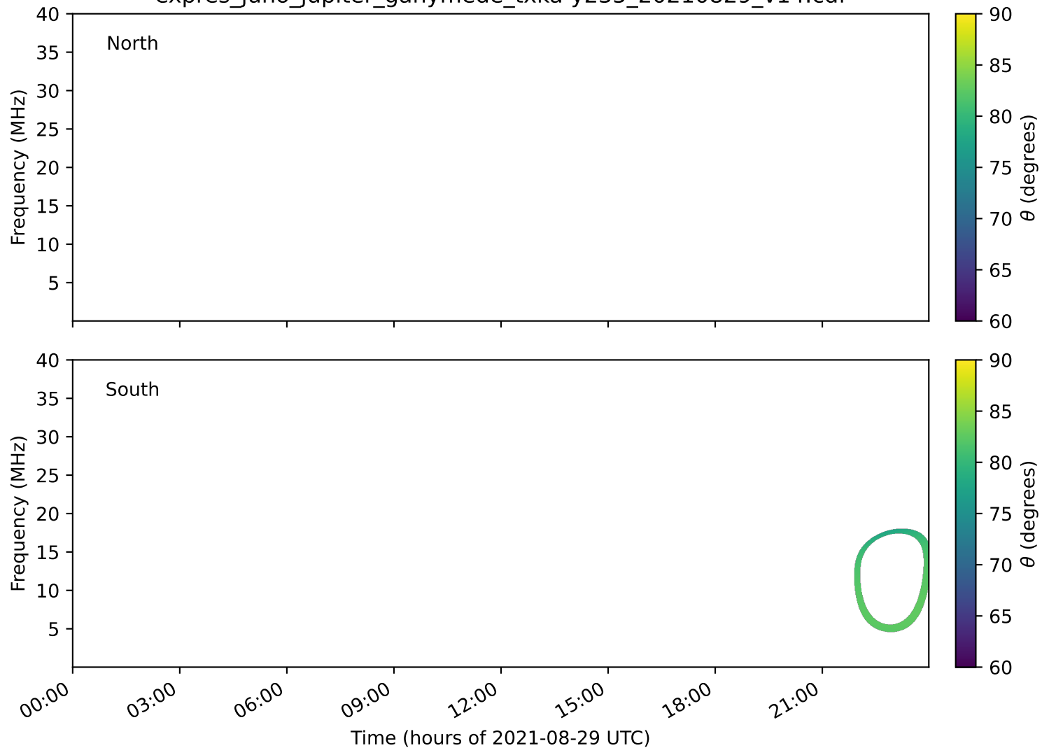
expres_juno_jupiter_ganymede_txka-y235_20210829_v14.cdf
