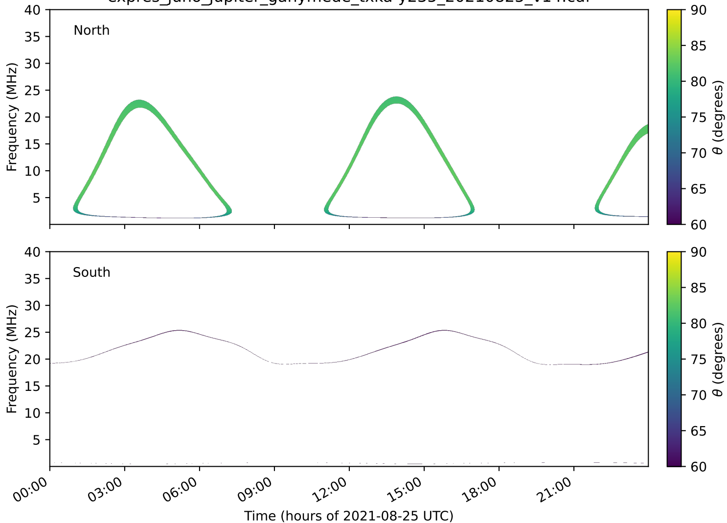
expres_juno_jupiter_ganymede_txka-y235_20210825_v14.cdf
