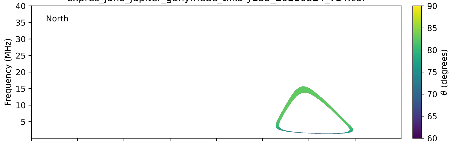
expres_juno_jupiter_ganymede_txka-y235_20210824_v14.cdf
