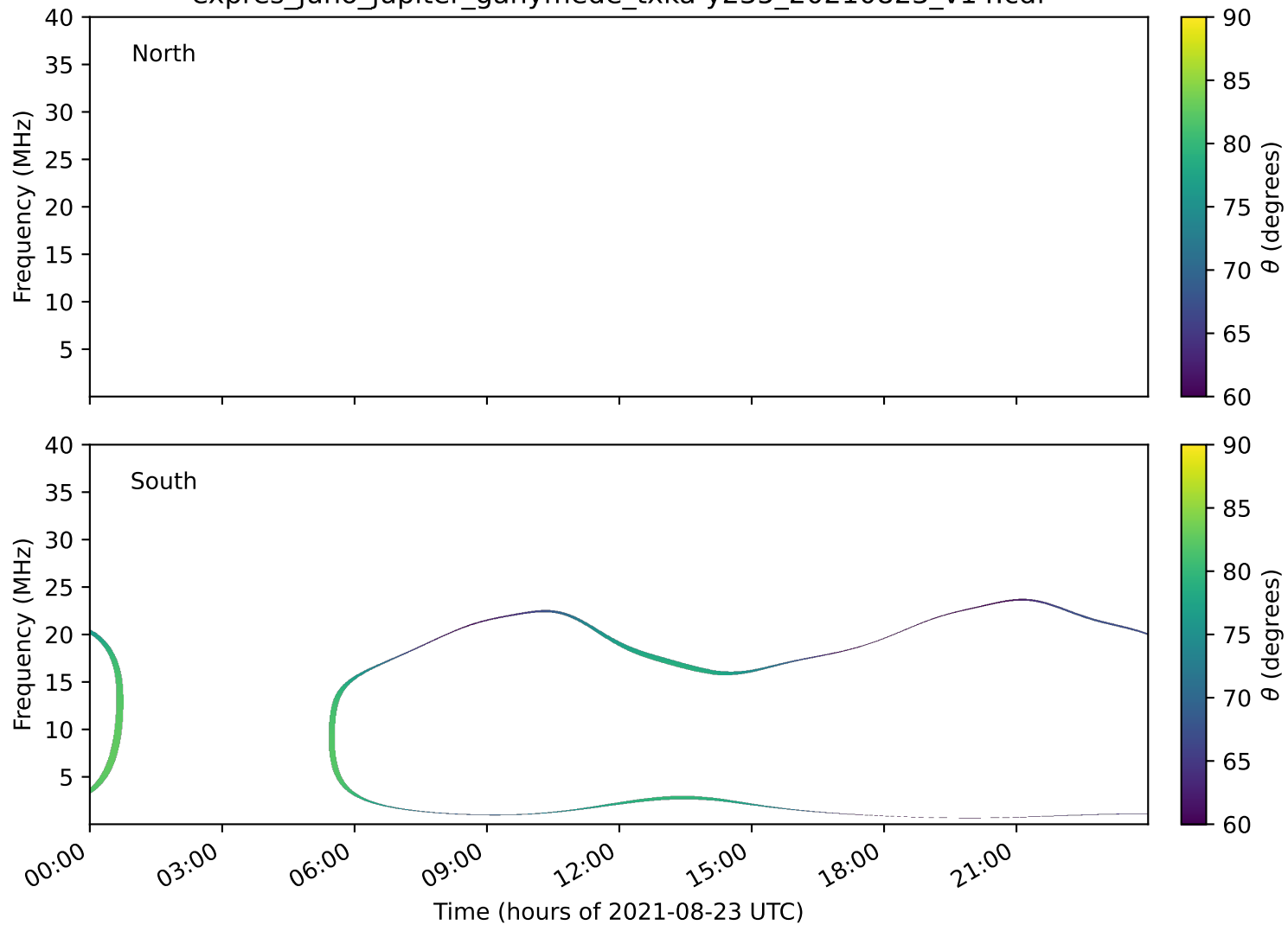
expres_juno_jupiter_ganymede_txka-y235_20210823_v14.cdf
