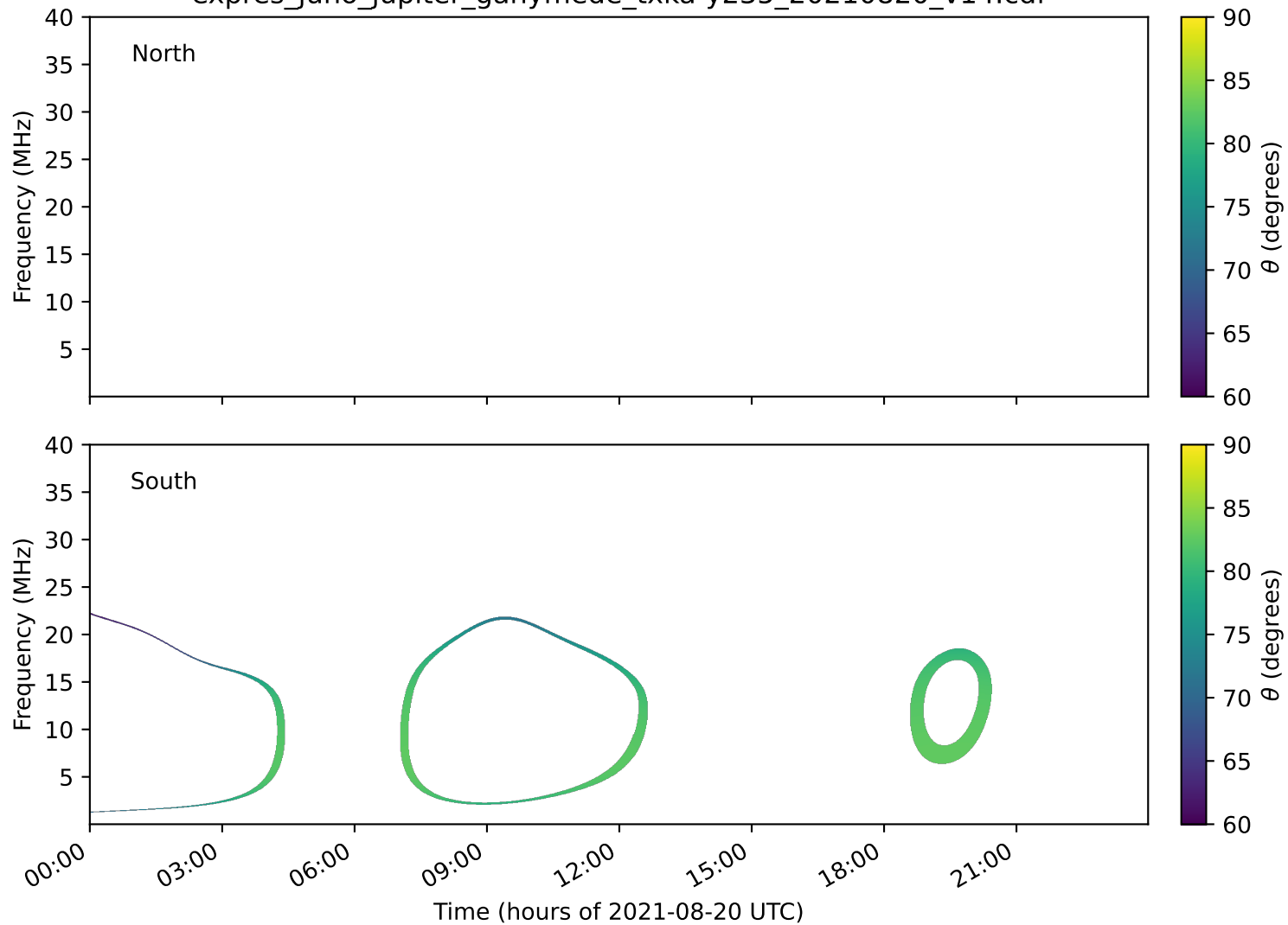
expres_juno_jupiter_ganymede_txka-y235_20210820_v14.cdf
